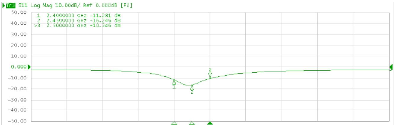
Figure 2. Antenna S-parameter
